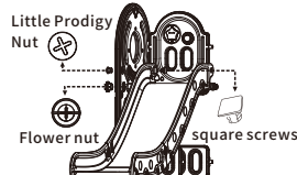
6 Fix the assembled slide to the large side panel
