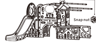
20 Insert the roof support rod into the corresponding hole in the roof
