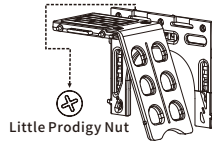
9 Climbing and fixing the assembled aisle platform strap to the U-shaped side panel of the aisle
