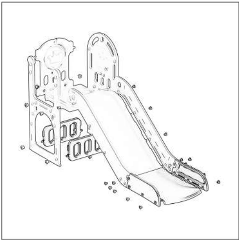
Step 2: Assemble the side plate, upper side plate, lower baffle, and platform with large nuts as shown in the figure. Then, use large nuts to assemble the slide tongue side plate and slide tongue of the slide, and connect the two with large nuts
