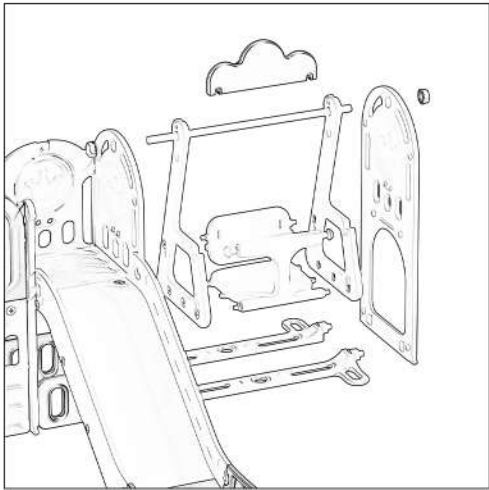
Step 4: Assemble the swing and connect it to one side of the slide with a nut
