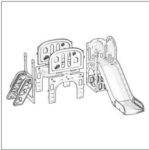
Step 3: Use large nuts to assemble the small aisle baffle, small aisle platform, large aisle baffle, large aisle platform, and large aisle arch as shown in the picture, and then connect the stairs and slides assembled in the first two steps
