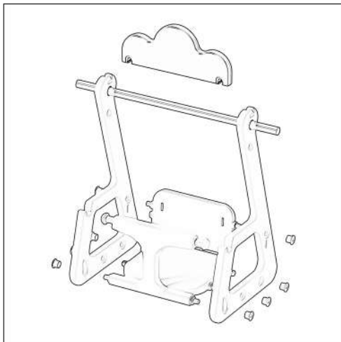
Step 4: Connect the swing side panel, swing front panel, and swing seat backrest with a large nut as shown in the picture
