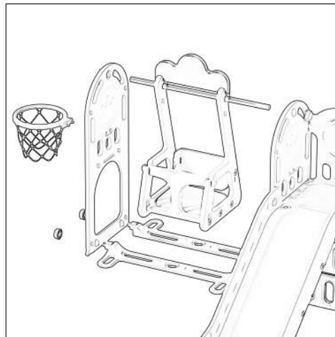
Step 5: Connect the crown side panel swing crossbeam swing base with a five corner nut and a large nut, then hang the swing onto the crossbeam with a rope, and assemble the basketball frame with a small nut
