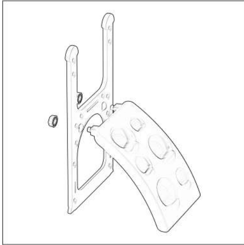
Step 1: Connect the climbing and U-shaped side panels with two hexagonal nuts as shown in the figure
